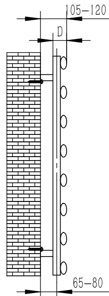
SIDE VIEW
