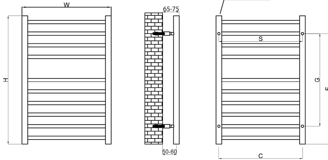
Front View
